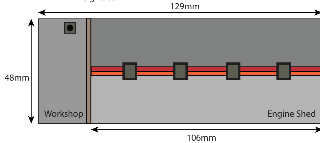
PN931/2 N Scale Single Track Engine Shed Height: 65mm
